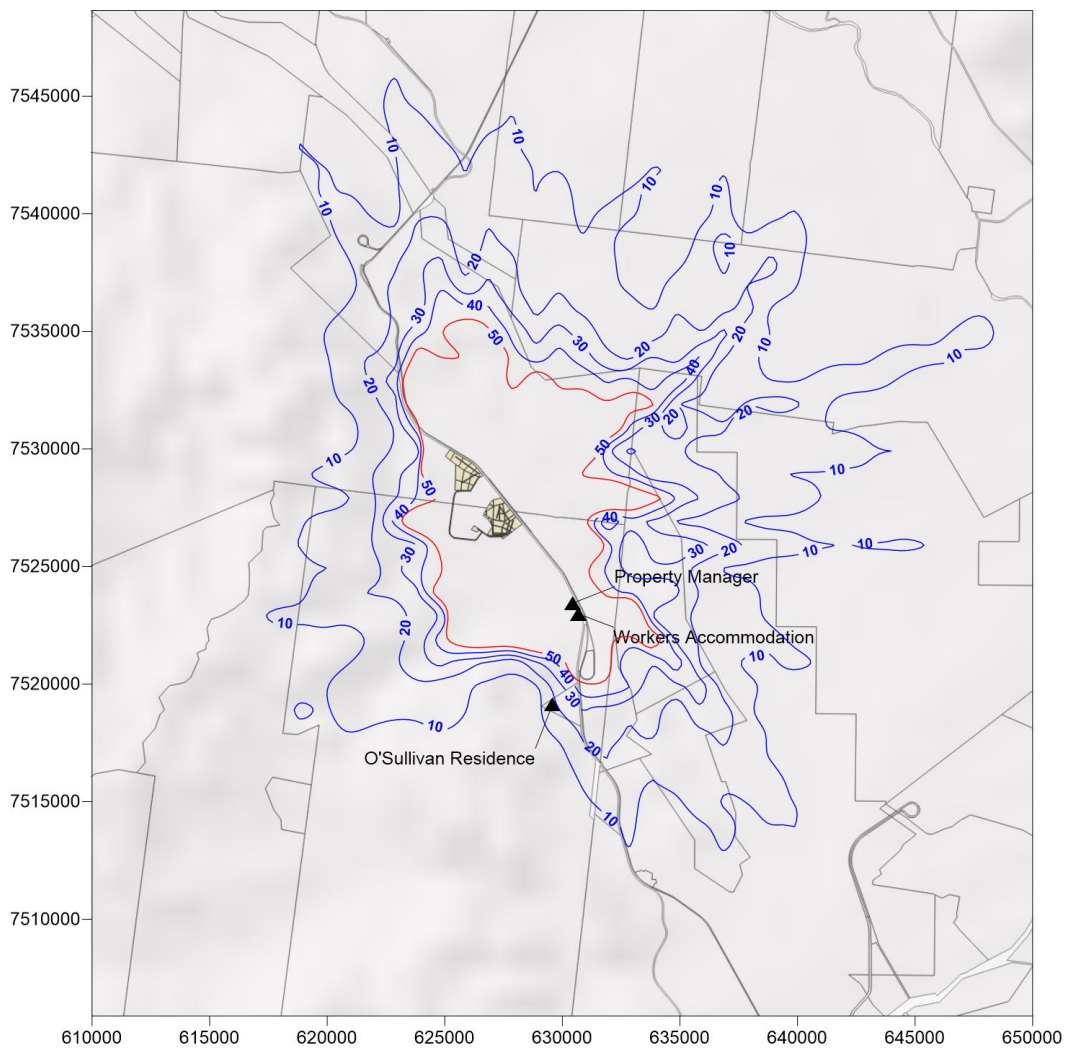
Plate 3 Predicted maximum 24-hour average ground-level concentrations of PM 10 for the VS Year 2 in isolation using standard mitigation measures
