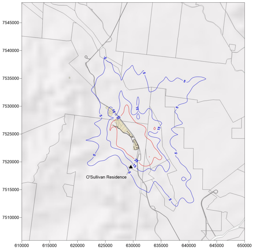
Plate 9 Predicted maximum 24-hour average ground-level concentrations of PM 2.5 for the VS Year 7 in isolation using standard mitigation measures
