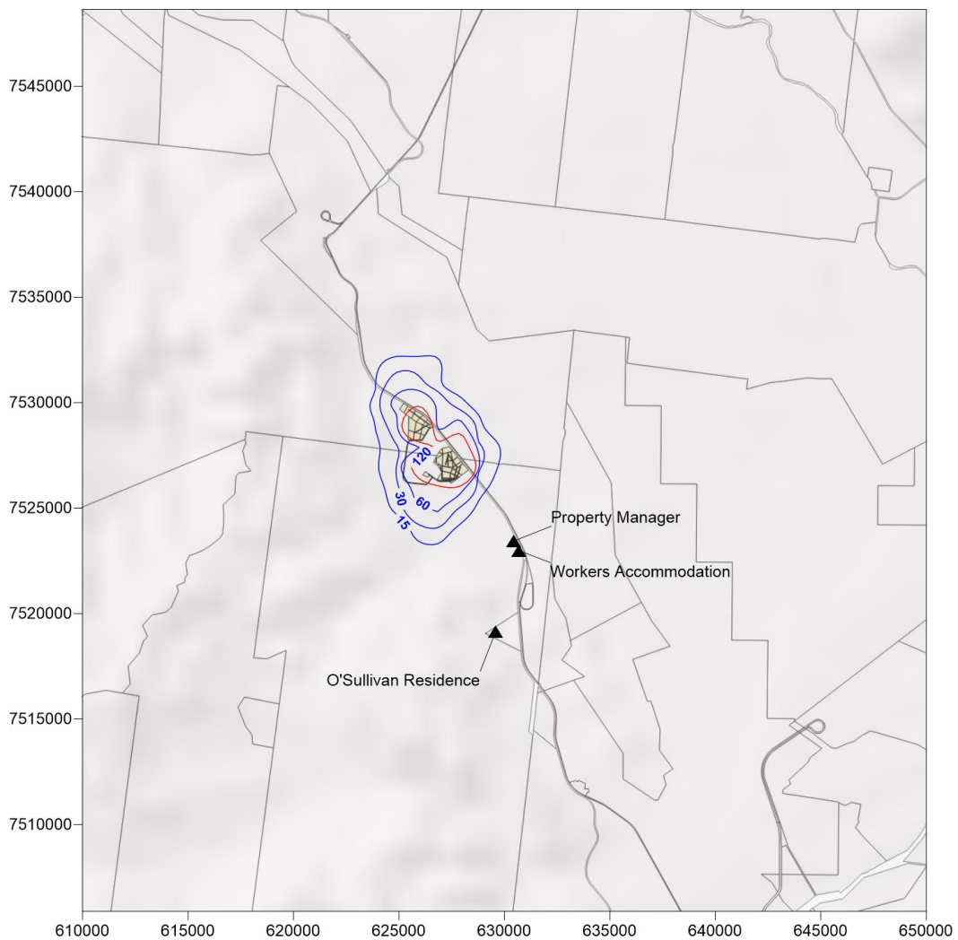
Plate 11 Predicted maximum monthly dust deposition rate for the VS Year 2 in isolation using standard mitigation measures
