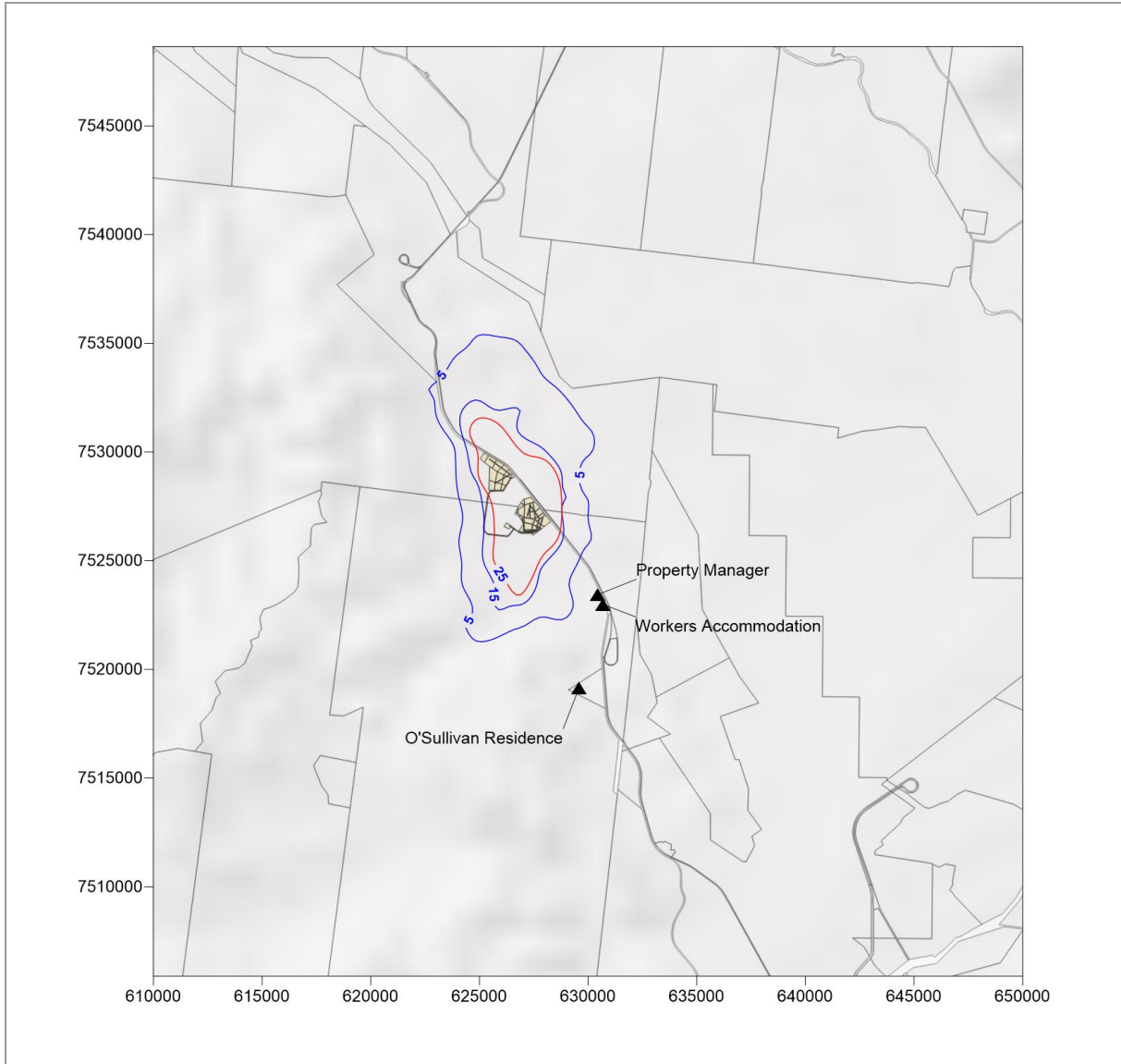
Plate 4 Predicted annual average ground-level concentrations of PM 10 for the VS Year 2 in isolation using standard mitigation measures
