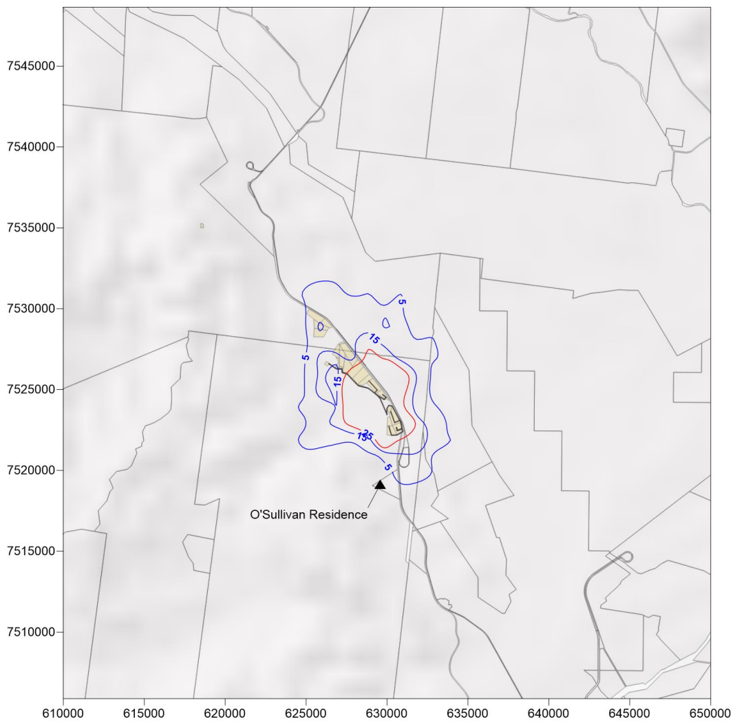
Plate 6 Predicted annual average ground-level concentrations of PM 10 for the VS Year 7 in isolation using standard mitigation measures
