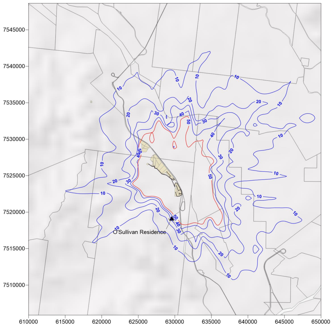
Plate 5 Predicted maximum 24-hour average ground-level concentrations of PM 10 for the VS Year 7 in isolation using standard mitigation measures
