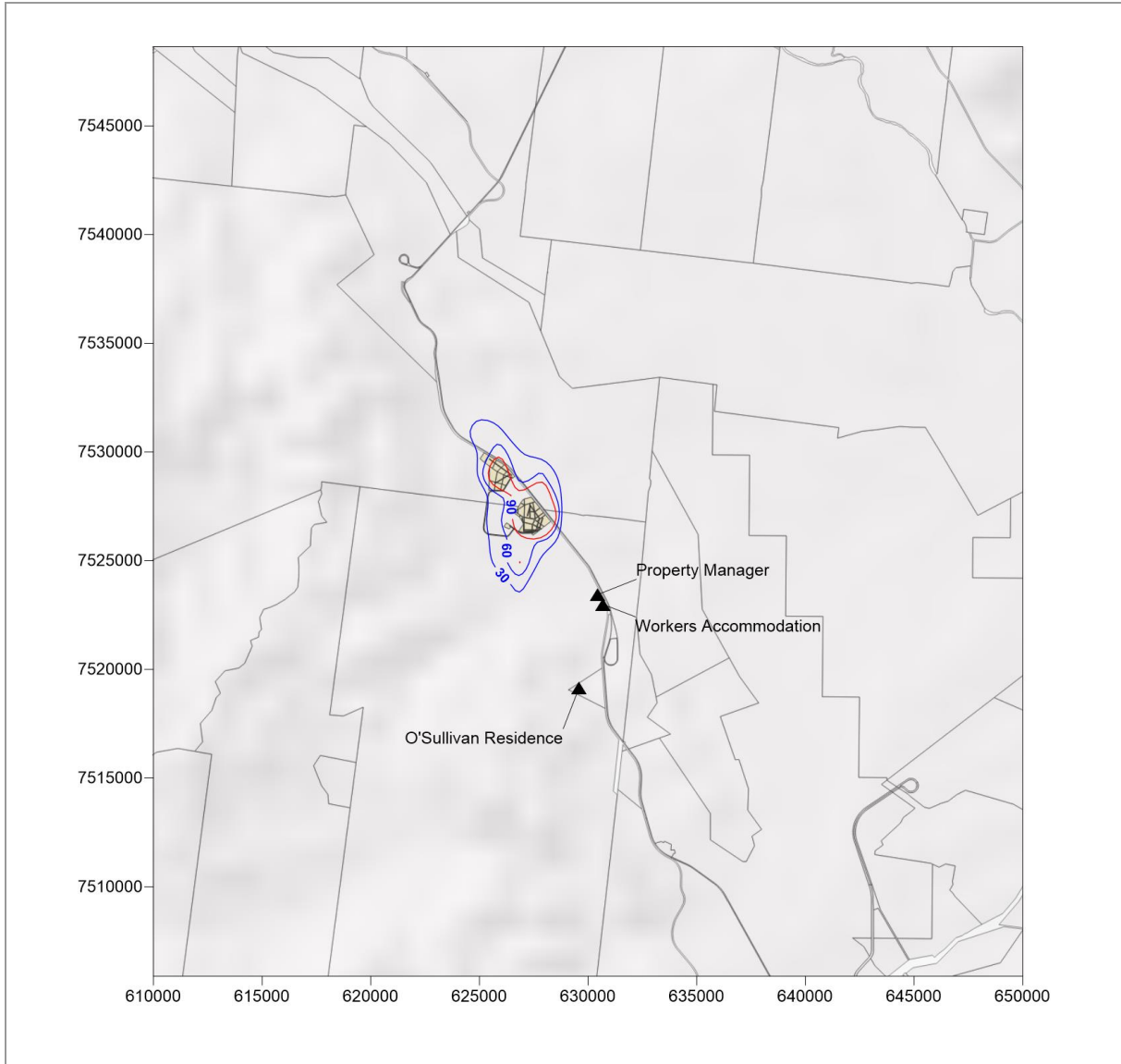
Plate 1 Predicted annual average ground-level concentrations of TSP for the VS Year 2 in isolation using standard mitigation measures
