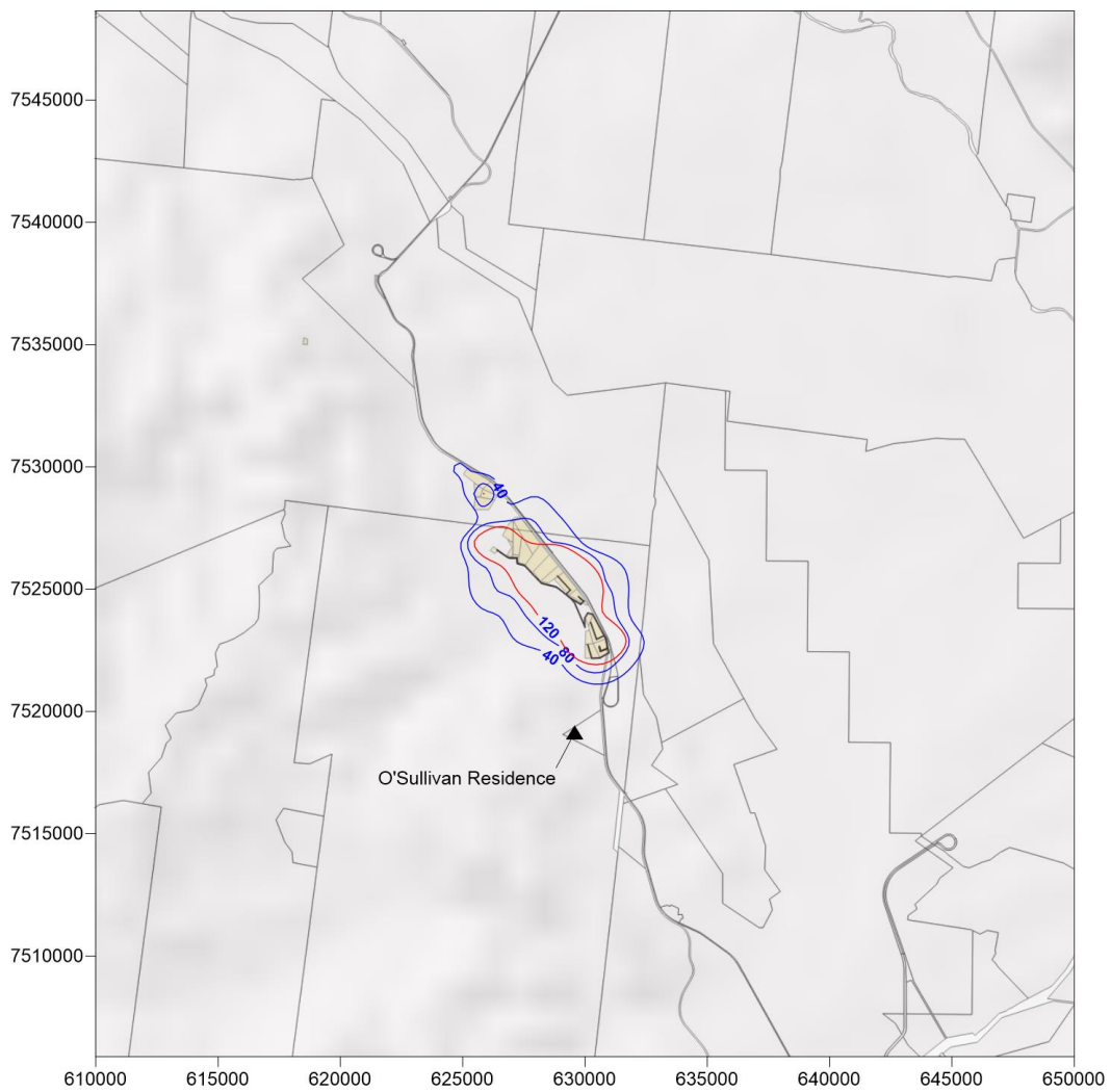
Plate 12 Predicted maximum monthly dust deposition rate for the VS Year 7 in isolation using standard mitigation measures
