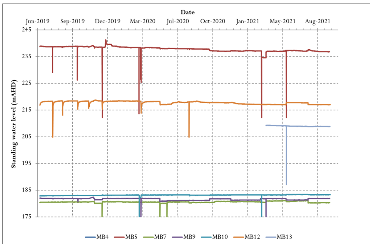
Figure 5.2 Groundwater hydrographs for Vulcan South monitoring bores
