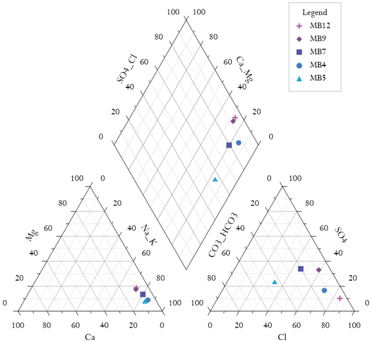
Figure 4.1 Piper diagram
