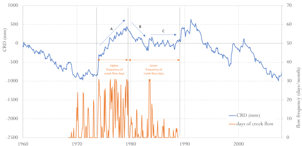
Figure 6 Frequency of creek flow compared to cumulative rainfall departure
