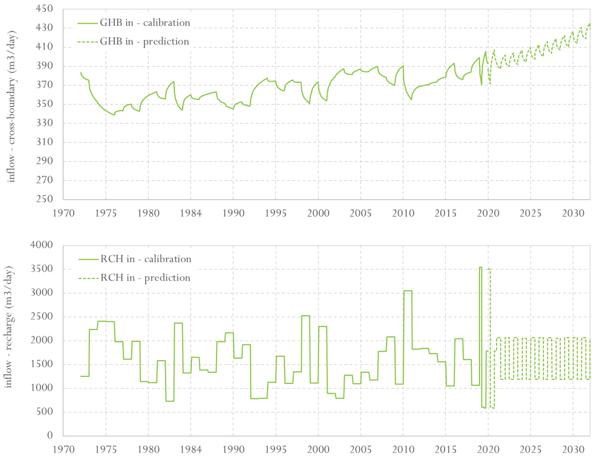
Figure 21 Numerical model budget – inflows (cross-boundary flow, rainfall related recharge)
