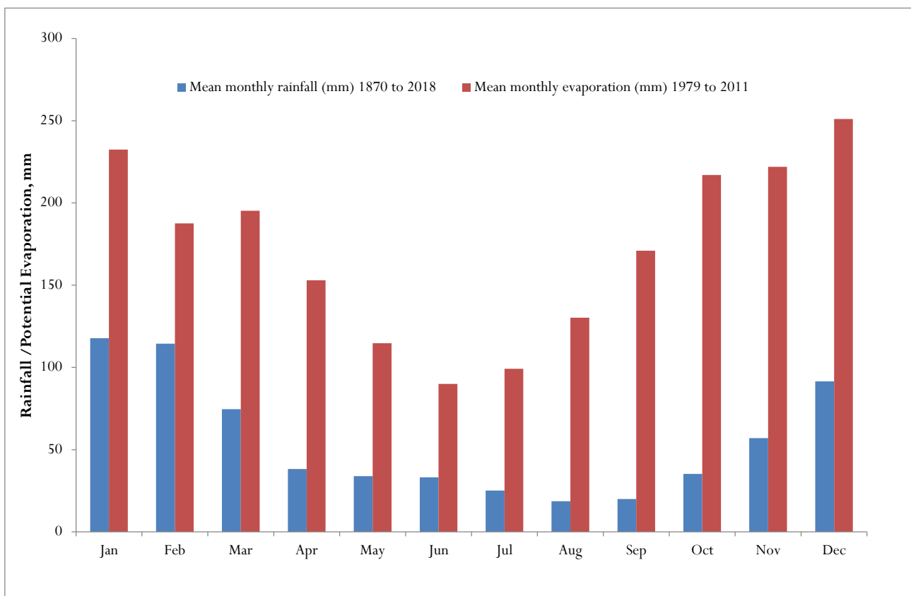
Figure 3.1 Rainfall and evaporation at Clermont Post Office (Station 035019)
