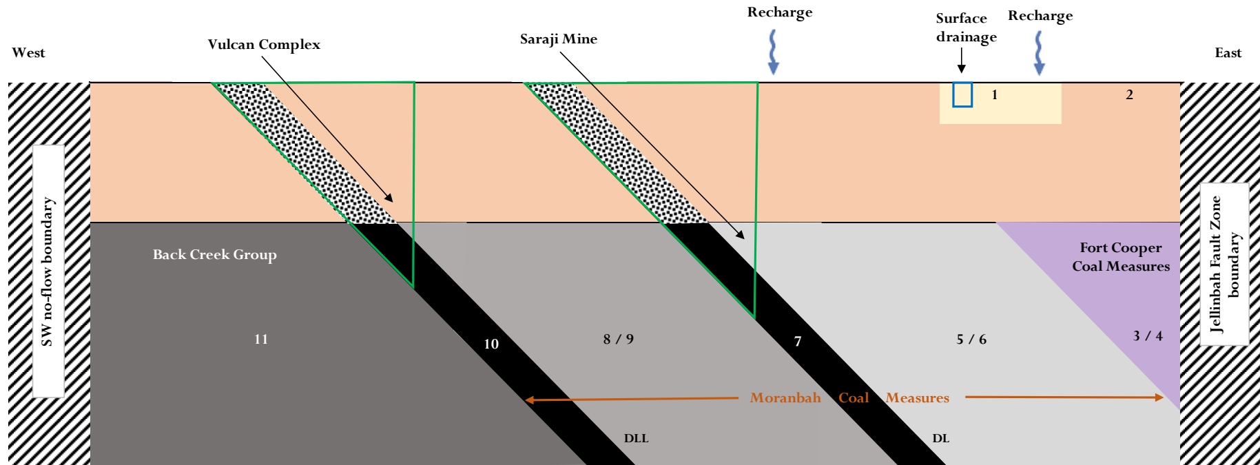
Figure 6.3 Model layers and boundary conditions
