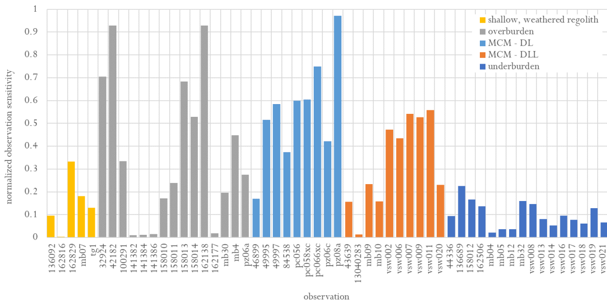
Figure 15 Normalised observation sensitivities
