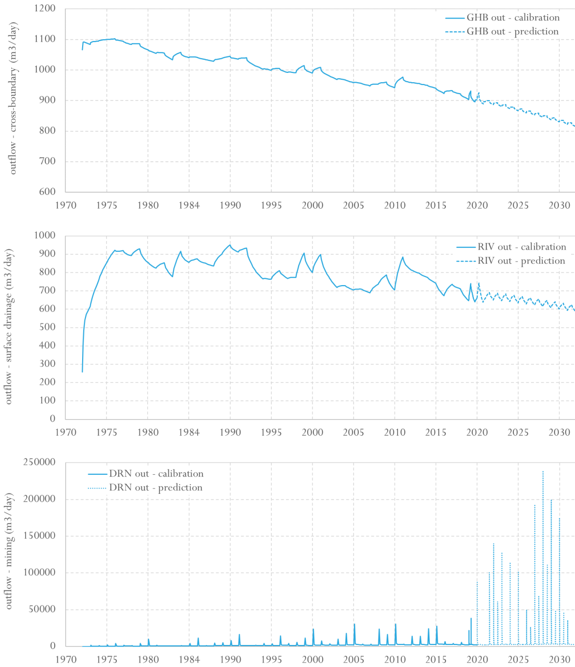
Figure 22 Numerical model budget – outflows (cross-boundary flow, surface drainage, mining)
