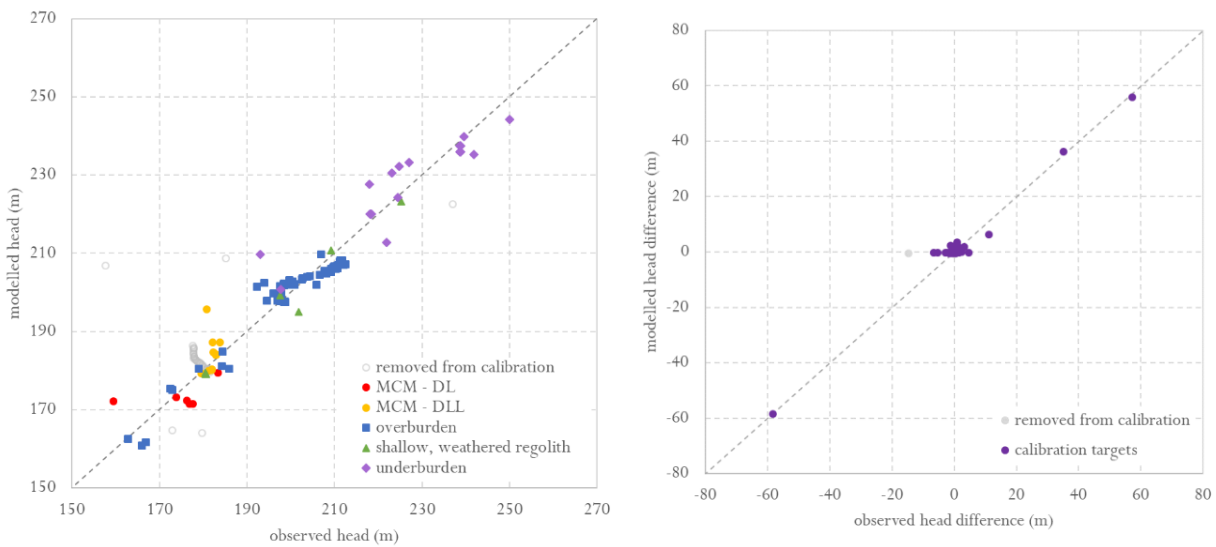
Figure 17 Model calibration scatter diagrams – observed and modelled heads and head differences
