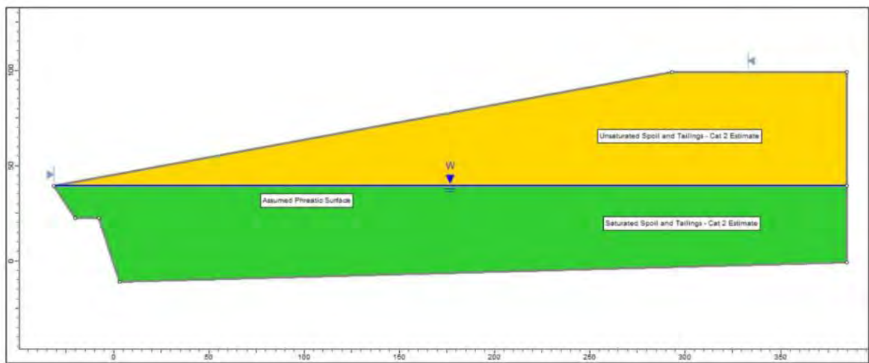
Figure 1-31 Geotechnical design of the in-pit spoil dumps of Vulcan South (Blackrock Mining Solutions Pty Ltd 2022)
