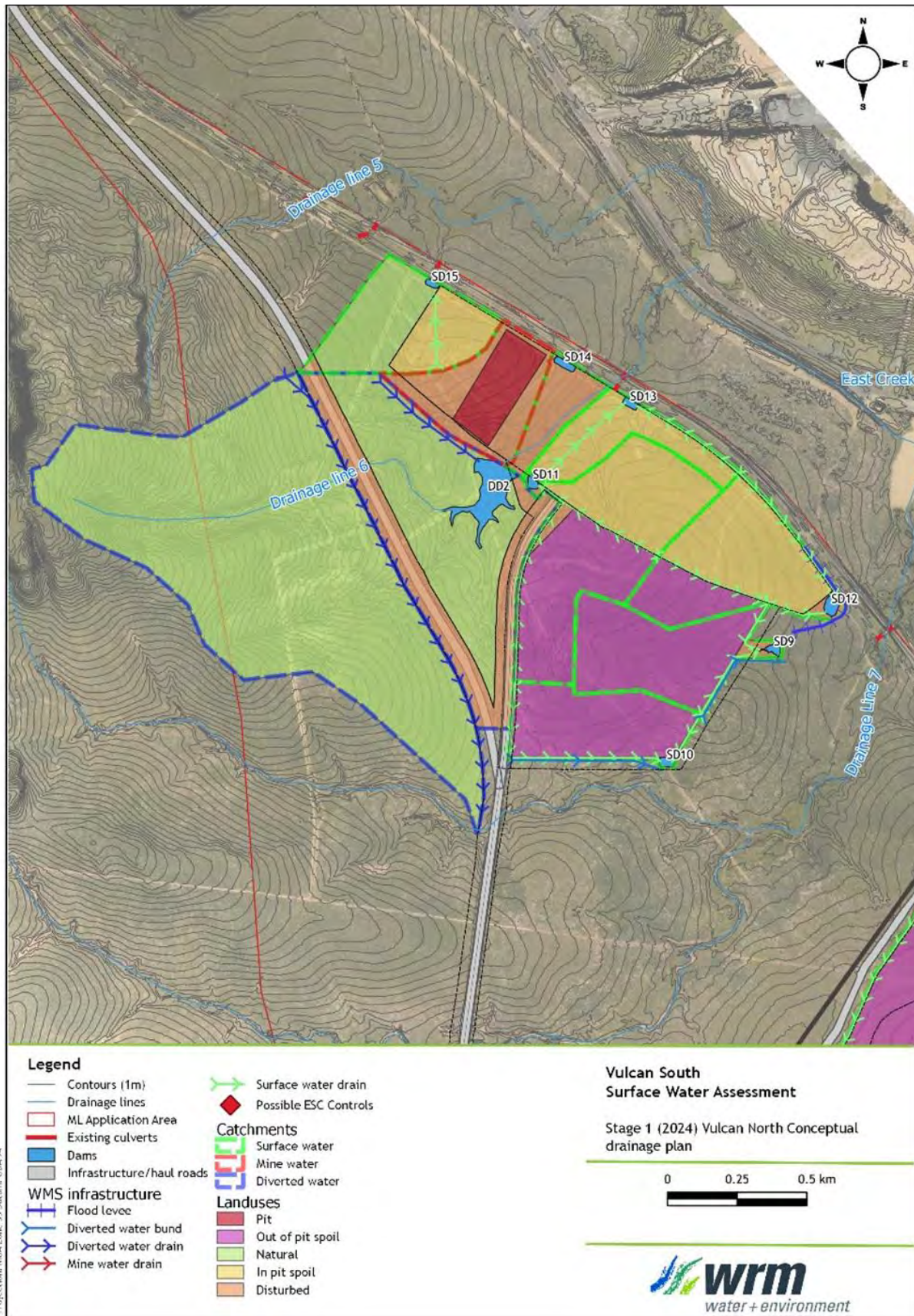
Figure 1-32 Stage 1 (Year 2024) Vulcan North mining area conceptual drainage plan
