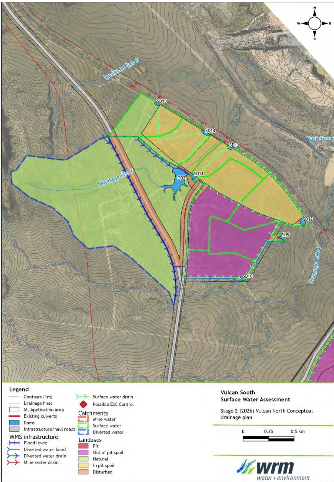
Figure 1-34 Stage 2 (year 2026) Vulcan North mining area conceptual drainage plan
