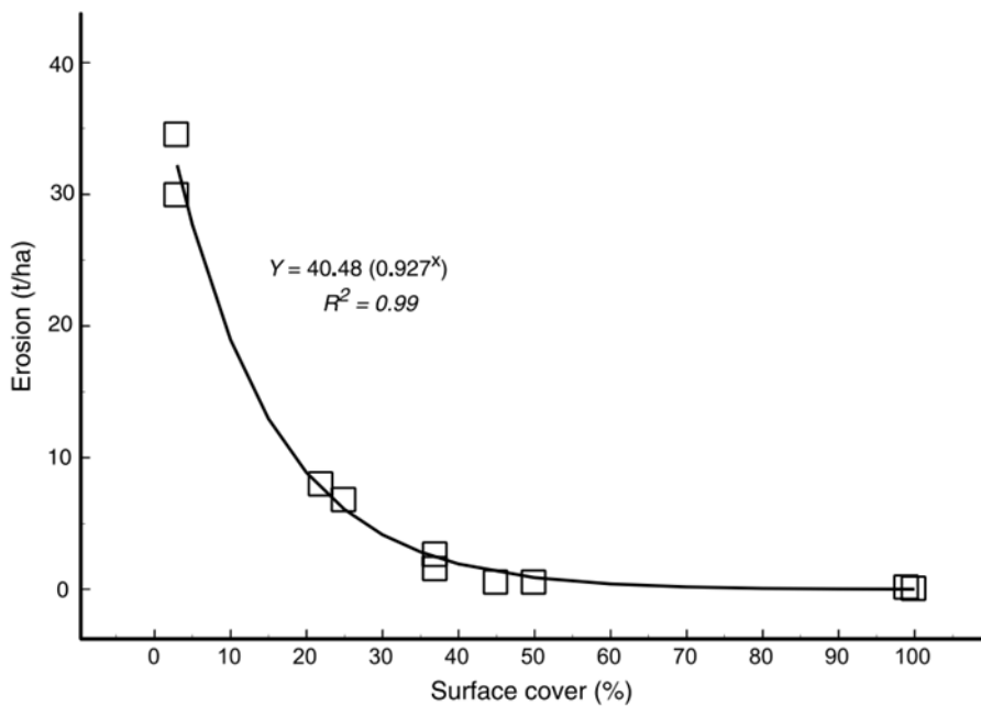
Figure 6-17 Effects of surface cover on erosion from 12-m-long plots with 15% slope under simulated rain at Tarong (figure from Loch 2000).
