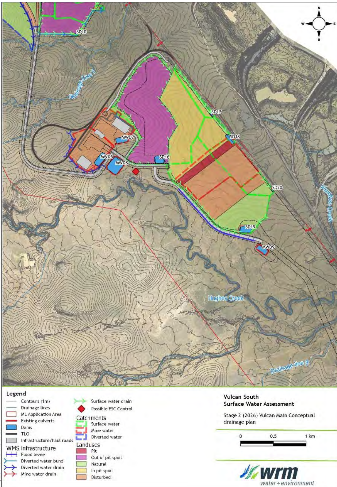
Figure 1-35 Stage 2 (year 2026) Vulcan Main mining area conceptual drainage plan
