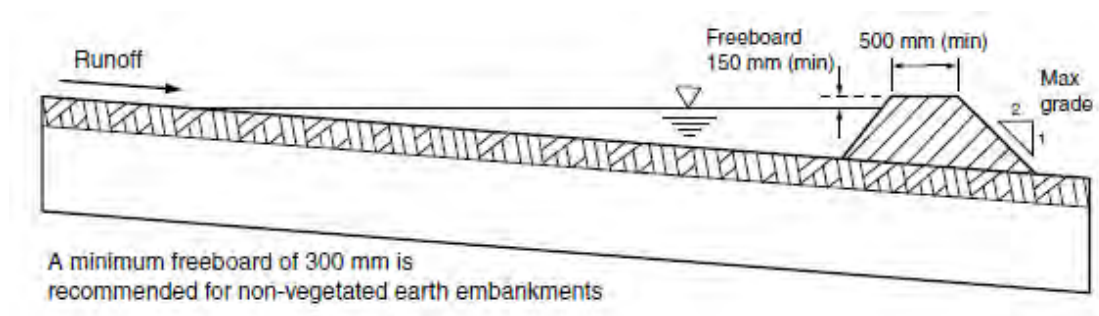
Figure 6.7 Upslope diverted water configuration – diversion bank (IECA, 2008)
